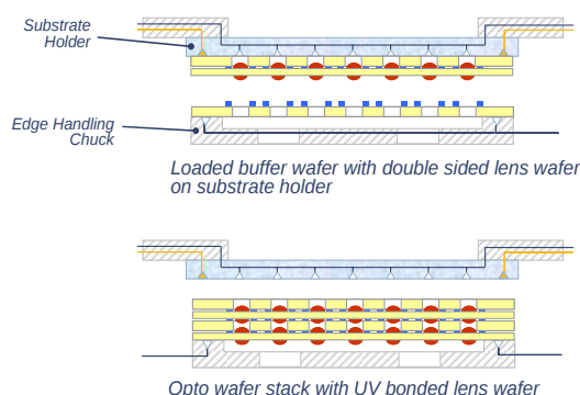
Figure 5: UV bonding incl. in-situ alignment on the SUSS MA8 Gen3 with the usage of buffer wafers
